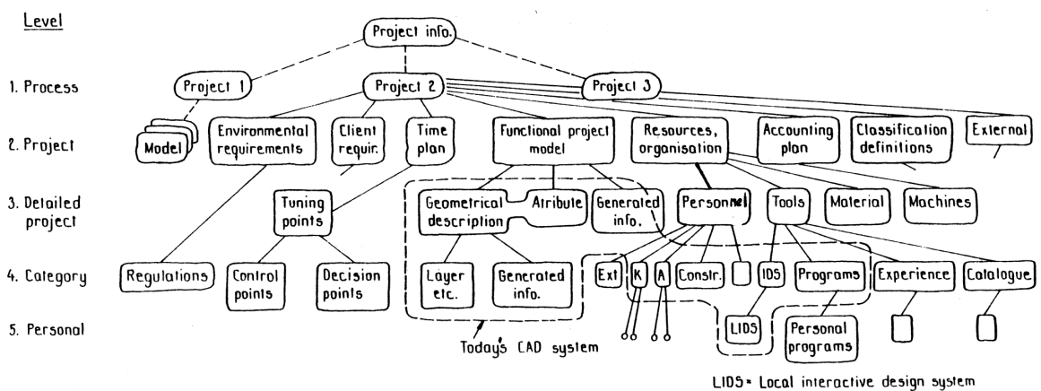
Figure 2 Process information and control structure, PICS
