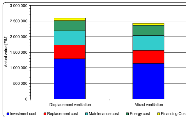
Figure 17. The building systems consultants projected the life-cycle costs of the displacement cooling and the mixed cooling options.
