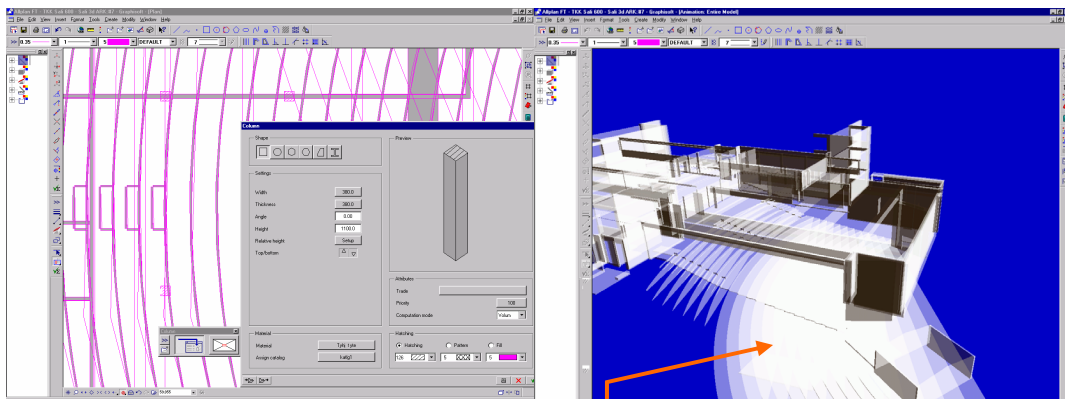
Figure 20. IFC import with distorted column and curvilinear geometries.
