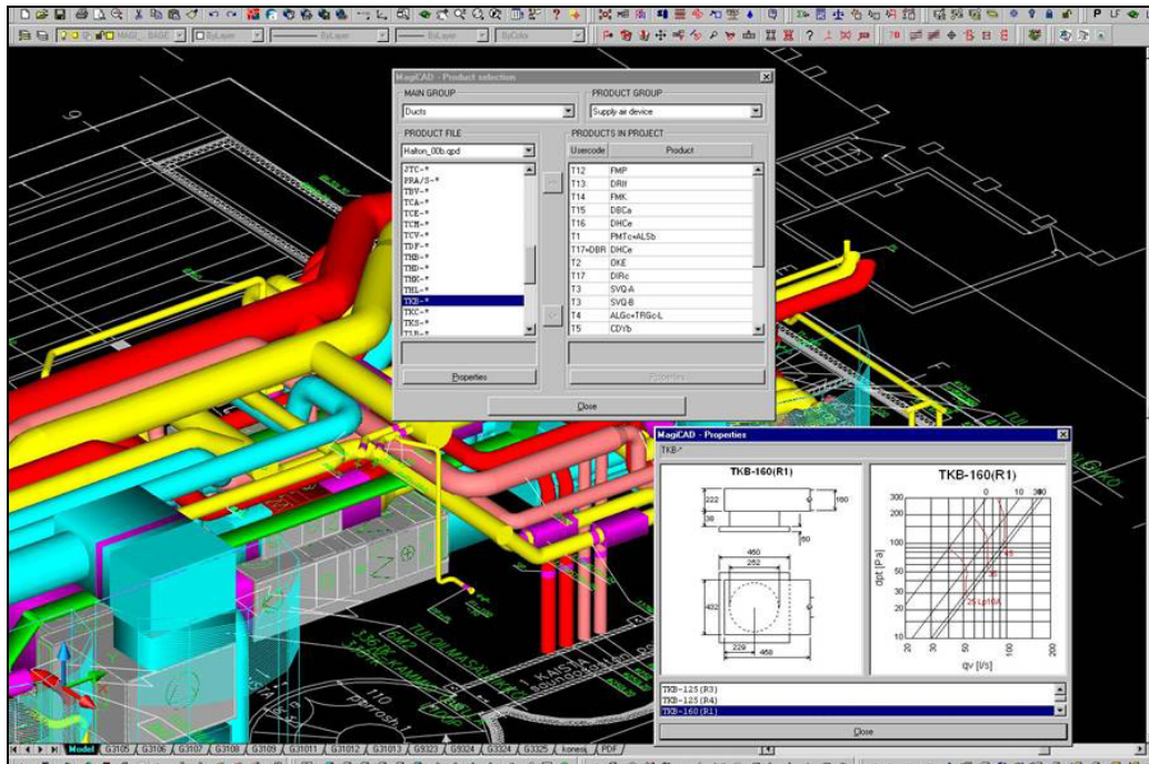
Figure 8: Granlund consultants used the 3D HVAC-CAD software MagiCAD to extract actual object information from the manufacturer's data.
