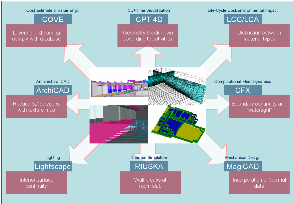
Figure 19: Domain-specific software applications (text in blue boxes) imposed different, and occasionally conflicting, input requirements (text in magenta boxes) onto the applications that generated a product model export for sharing.
