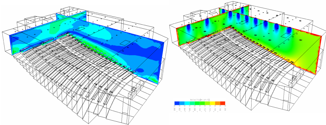
Figure 12. CFX provided CFD cross-sectional profiles of air velocity in the displacement cooling scenario (left) as well as the mixed cooling scenario (right).
