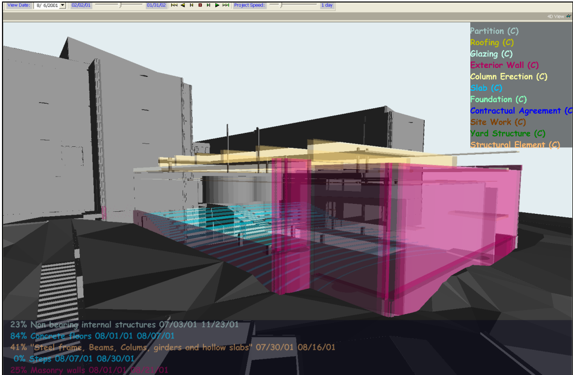
Figure 16. A view from the HUT-600 4D model highlighting the different construction activities that are scheduled to take place on a particular date.
