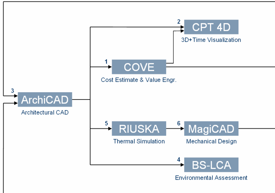
Figure 10. Flow of IFC files across software applications and disciplines on the HUT-600 project.
