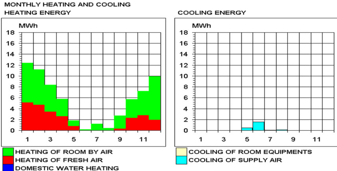
Figure 11. RIUSKA projected the annual heating and cooling energy consumption for HUT-600.
